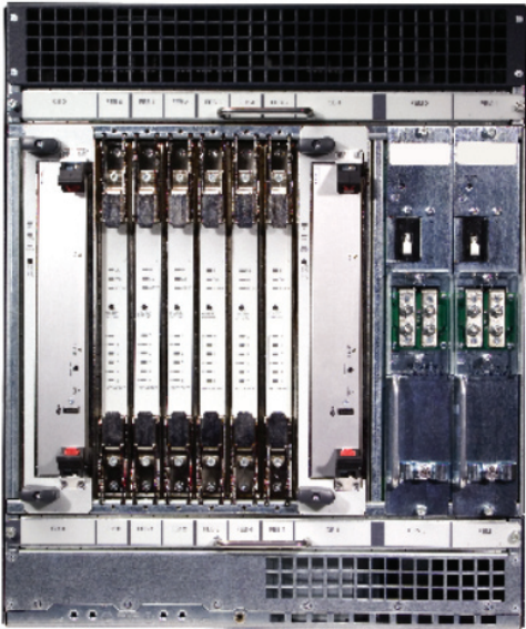
Six rear-mounted Forwarding Engine Boards (FEBs) supply redundant forwarding capability to all PICs installed in the chassis without requiring standby interface modules.
